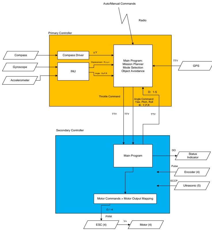
Figure 6: Phase 2 Control System
