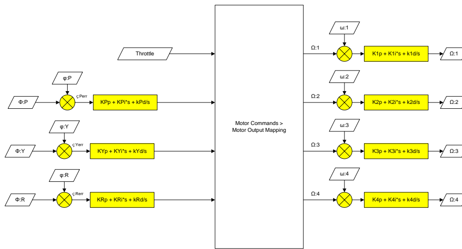
Figure 10: Phase 3 Secondary Controller Block Diagram
