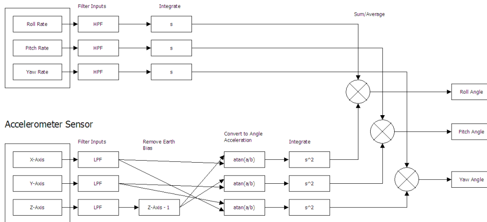
Figure 11: INU Diagram
